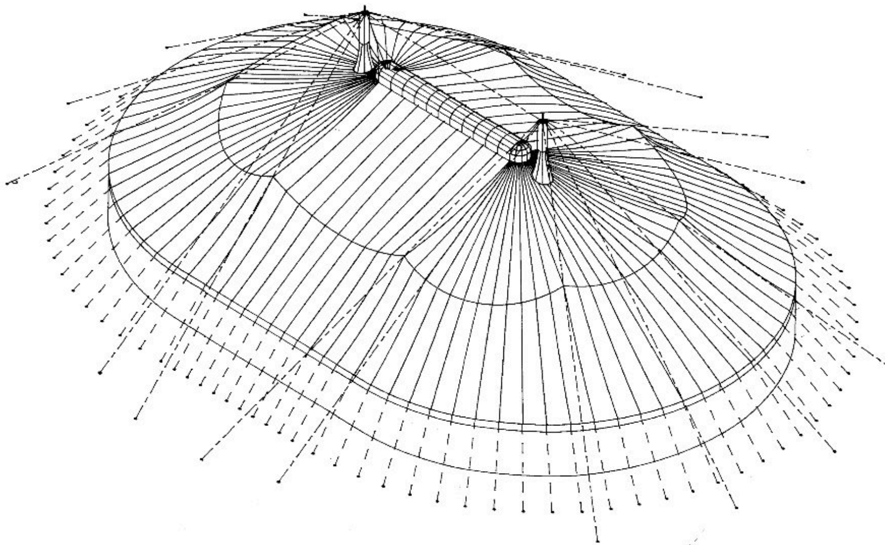
ISOMETRIC VIEW
